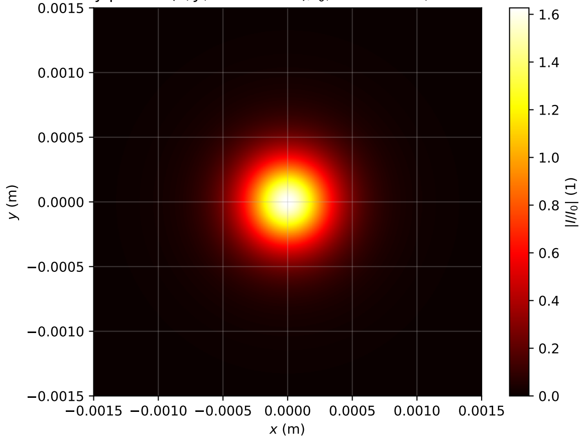
Intensity profile I(x, y, z = 1.911m)/I_0 , \text{Pin}=0.9\text{Pcr} , artificial time
